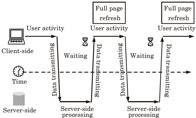
Fig. 3.15.1. Traditional web application communication flow.
