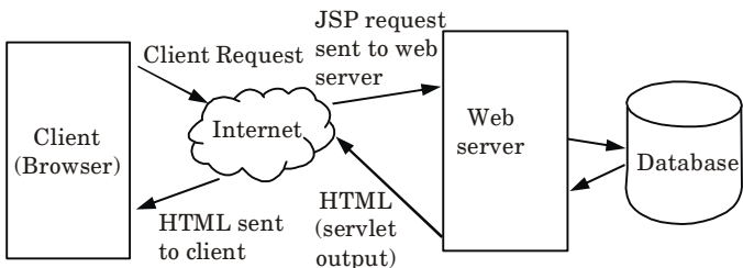
Fig. 5.16.1. JSP architecture.
