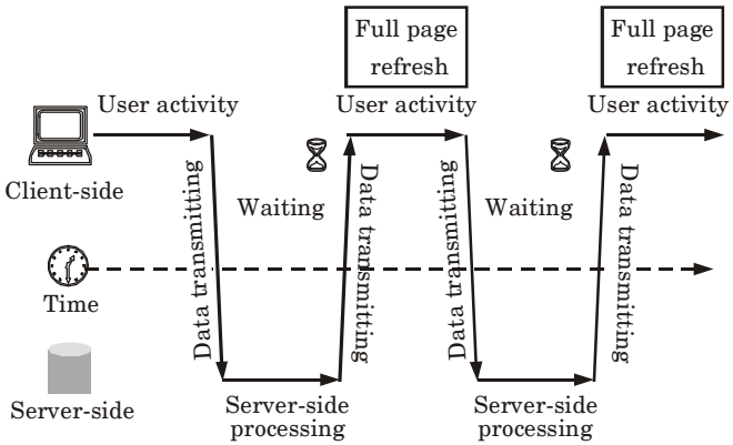
Fig. 1 Traditional web application communication flow.
